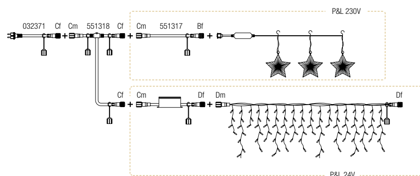
EXAMPLE OF MIXED 230V AND 24V WIRING
