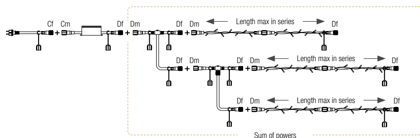
EXAMPLE OF SERIES AND PARALLEL WIRING
